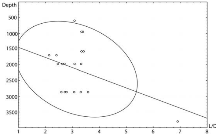
Fig. 10. Changes of L/D ratio with depth in Bathycrinus carpenteri .
