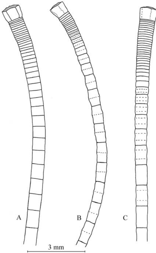
Fig. 9. Variation of the form of columnals in proxistele and upper mesistele in Bathycrinus carpenteri (M. Sars 1900, St. 9, depth 1960 m).
